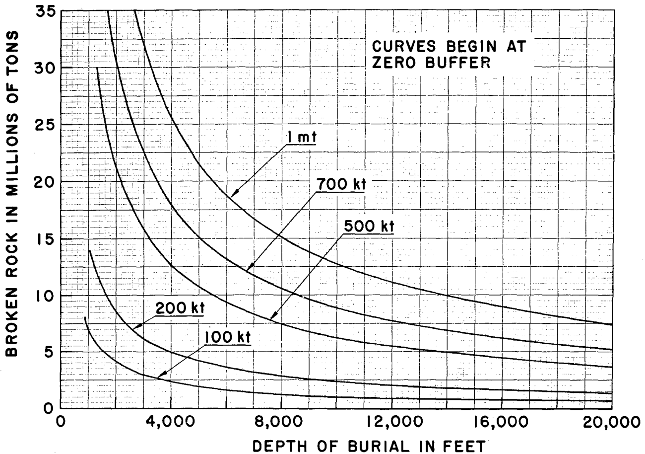
Fig. 4. Tonnages of granitic rock broken by underground nuclear explosions (50 kt).
